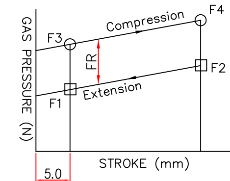
GAS PRESSURE DIAGRAM
