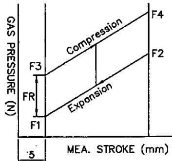
GAS PRESSURE DIAGRAM
