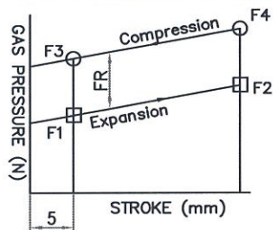
GAS PRESSURE DIAGRAM
