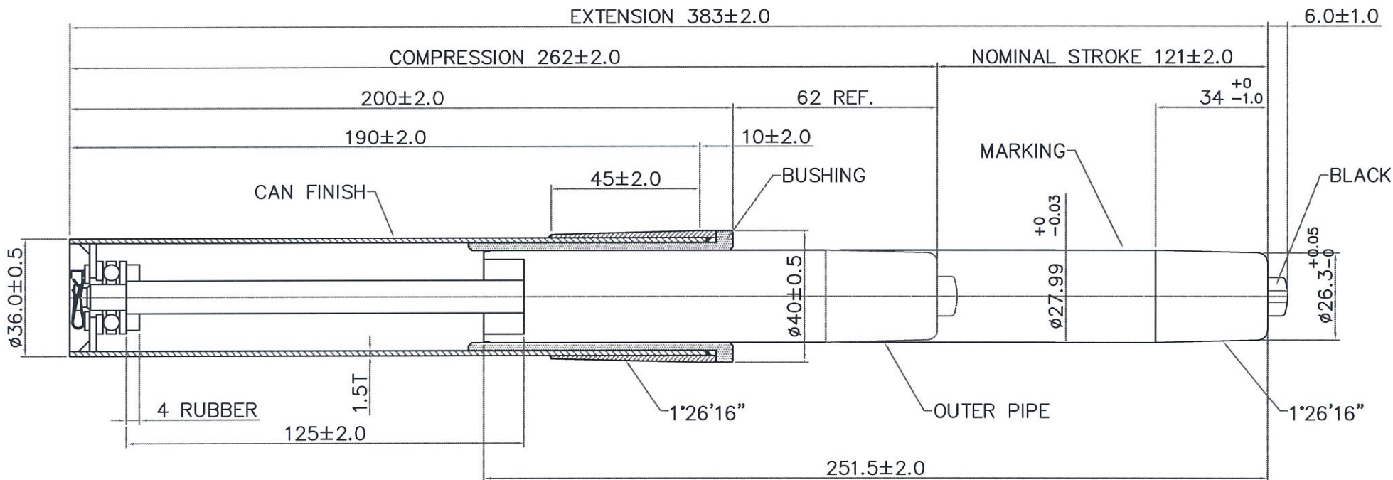
GAS PRESSURE DIAGRAM
