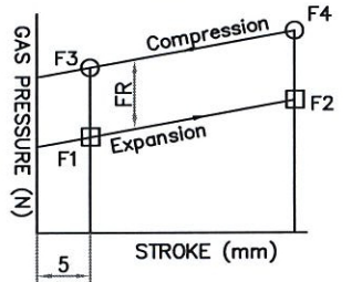
GAS PRESSURE DIAGRAM
